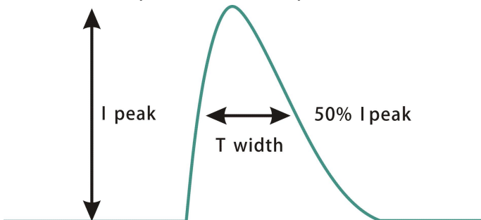
Inrush current(DL-80H-GX-MXK)
