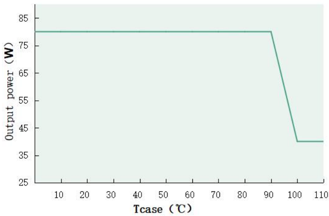
Output power VS Tcase (DL-80H-GX-MXK)
