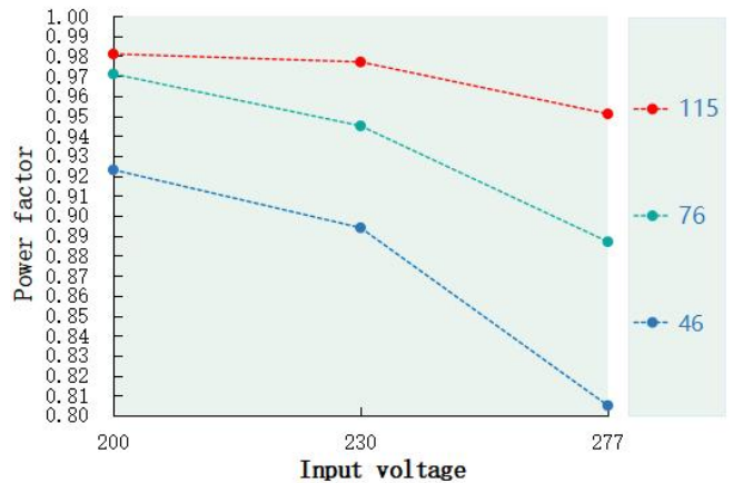
Power factor VS Input voltage(DL-80H-V115GX-MXK)
