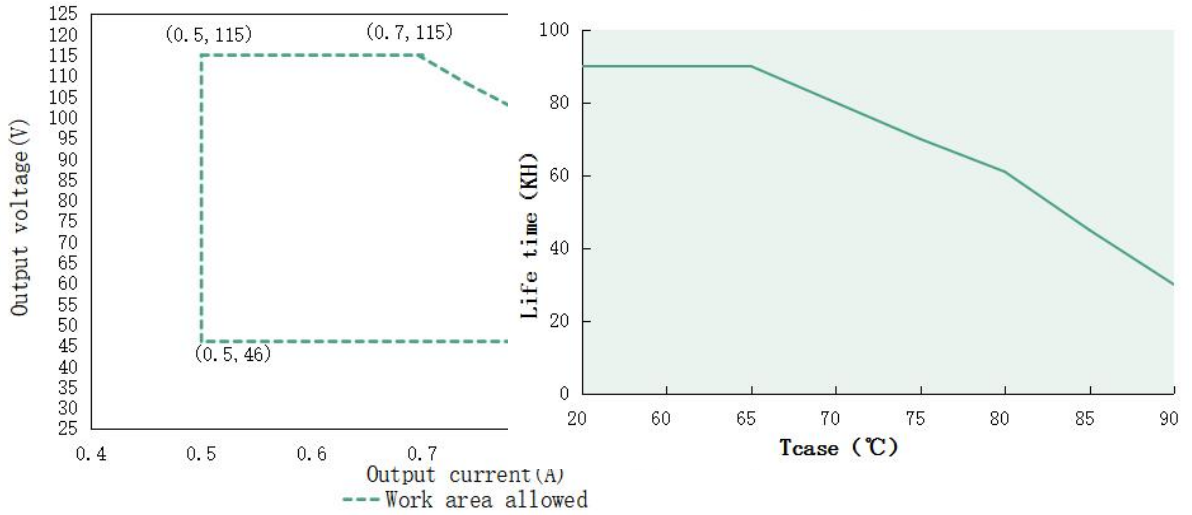
Output voltage VS output current of DL-80H-V115GX-MXK (input: 200-277Vac)
