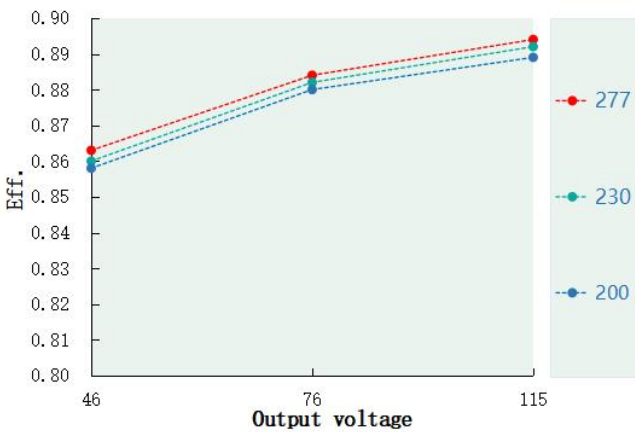
Eff. VS Output voltage(DL-80H-V115GX-MXK)
