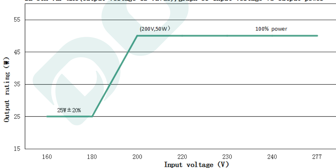
DL-50H-72P-MXC(When the output voltage is 72Vdc, the rated output current value and output power corresponding to different input voltage)
