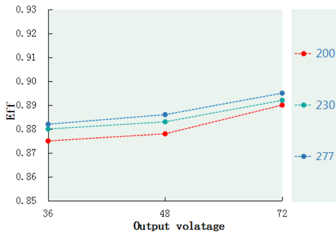
Eff. VS Output voltage(DL-50H-V72P-MXC)
