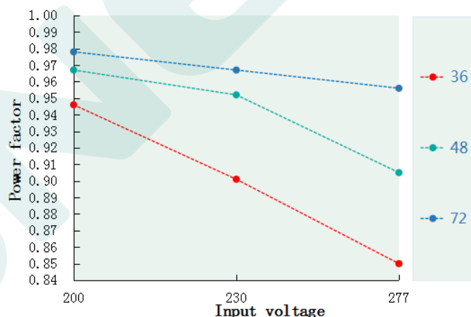
Power factor VS Input voltage(DL-50H-V72P-MXC)
