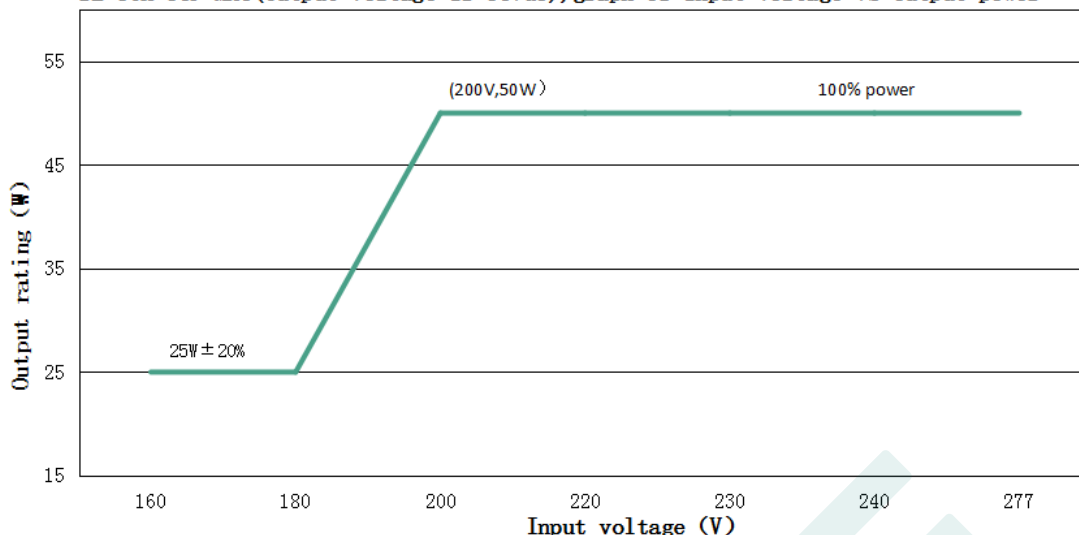
DL-50H-56P-MXC(When the output voltage is 56Vdc, the rated output current value and output power corresponding to different input voltage)
