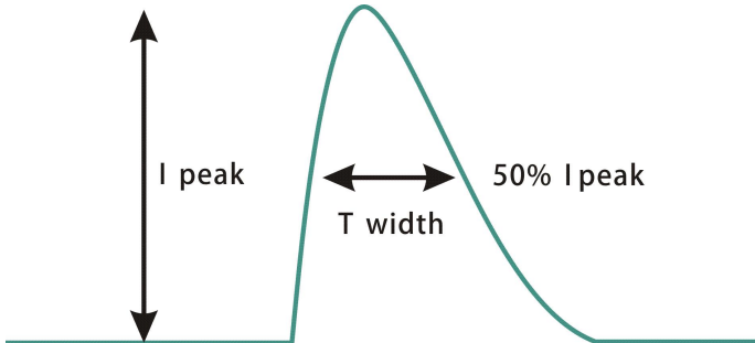
Inrush current(DL-40H-GX-MXK)
