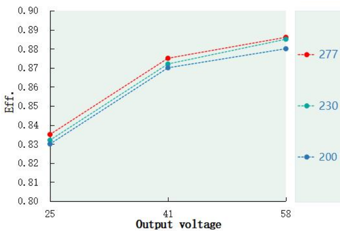
Eff. VS Output voltage(DL-40H-V58GX-MXK)
