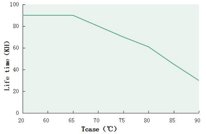
Tcase VS Lifetime (DL-40H-GX-MXK)
