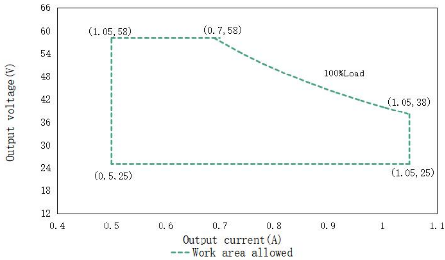
Output voltage VS output current of DL-40H-V58GX-MXK (input: 200-277Vac)
