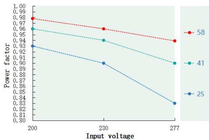
Power factor VS Input voltage(DL-40H-V58GX-MXK)
