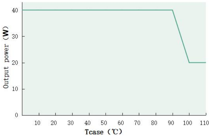
Output power VS Tcase (DL-40H-GX-MXK)
