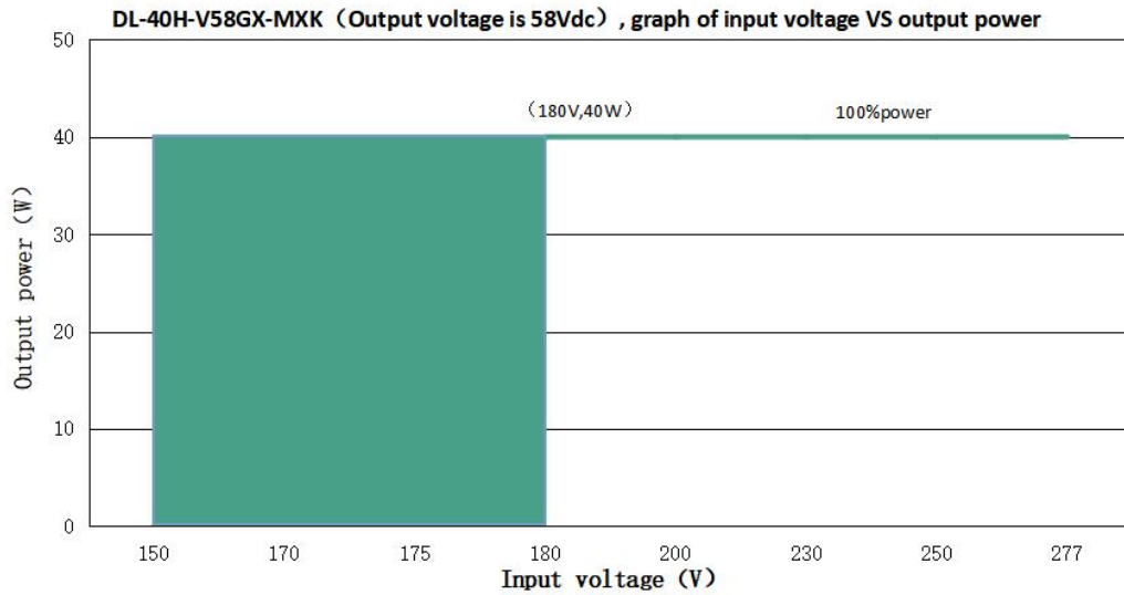
DL-40H-V58GX-MXK (When the output voltage is 58Vdc, the rated output current value and output power corresponding to different input voltage)
