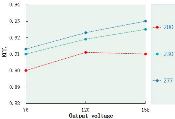
Eff. VS Output voltage(DL-110H-V158GX-MXK)
