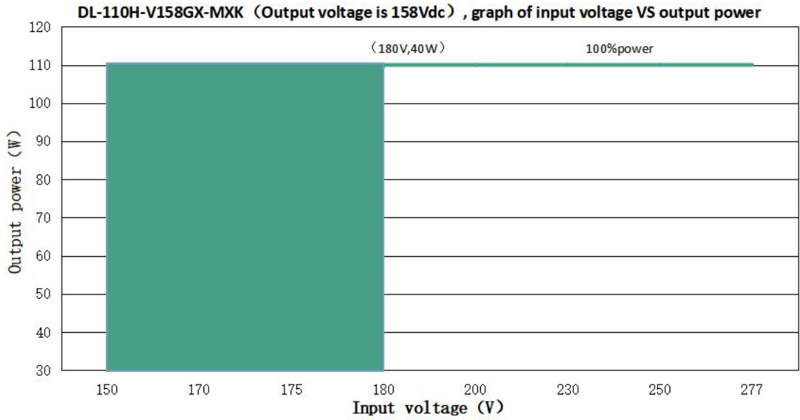
DL-110H-V158GX-MXK (When the output voltage is 158Vdc, the rated output current value and output power corresponding to different input voltage)
