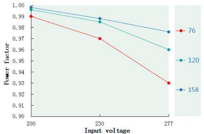
Power factor VS Input voltage(DL-110H-V158GX-MXK)
