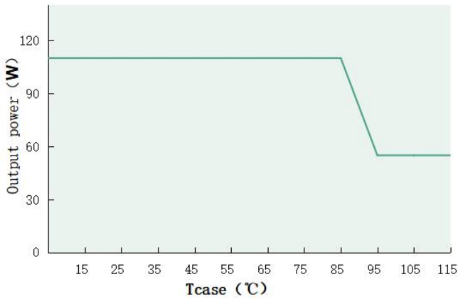
Output power VS Tcase (DL-110H-GX-MXK)
