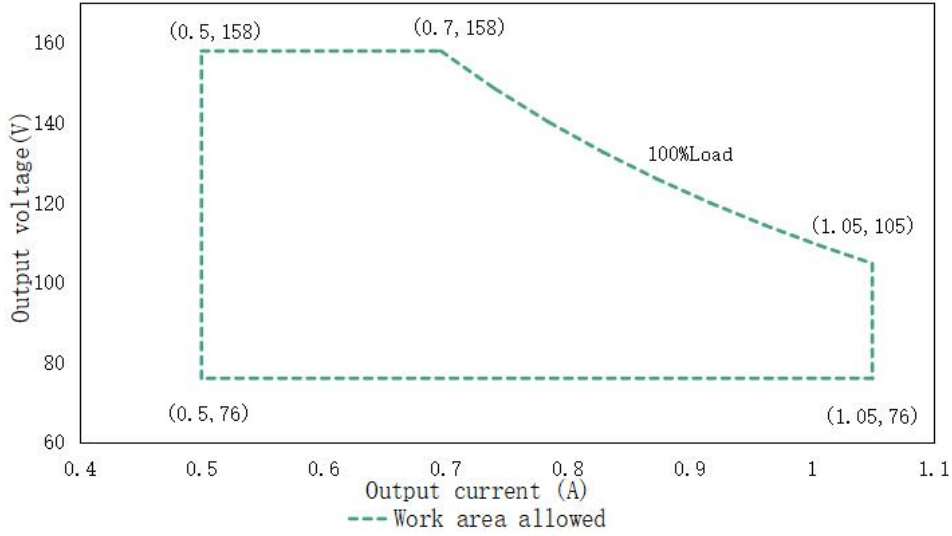
Output voltage VS output current of DL-110H-V158GX-MXK (input: 200-277Vac)
