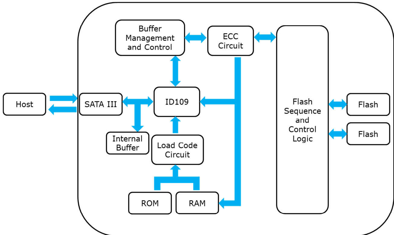
Figure 2: Innodisk CFast 3IE3 Block Diagram
