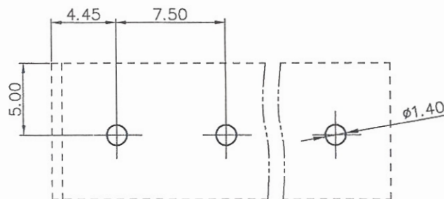
PCB LAYOUT
