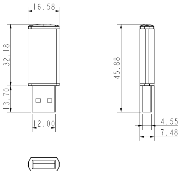
Figure 3: USB Drive 2SE mechanical dimensions
