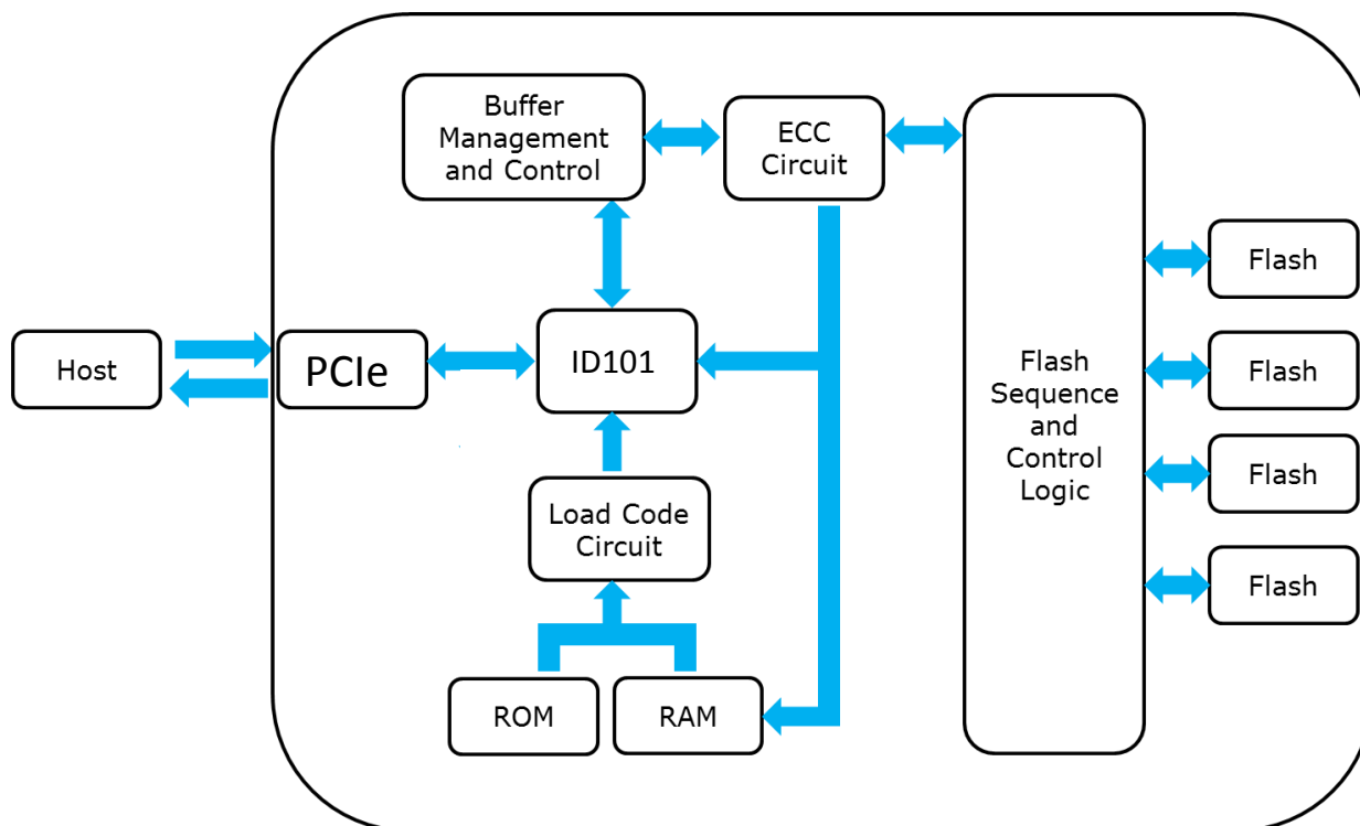
Figure 2: Innodisk Mini PCIeDOM 1SE Block Diagram
