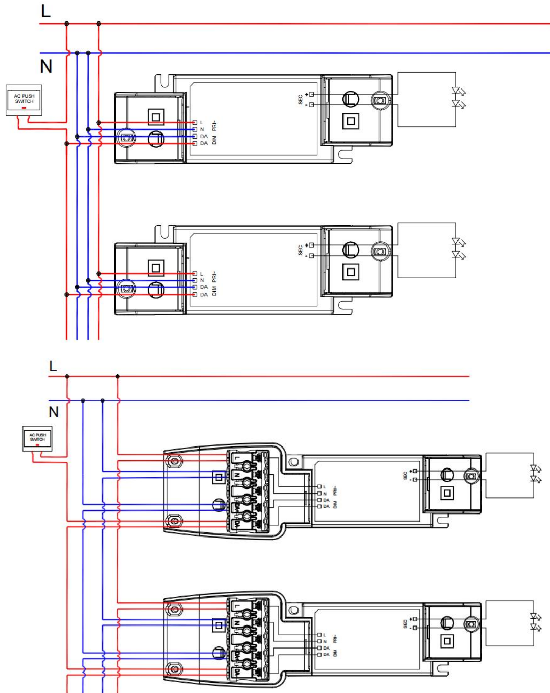
Fig. B: Push Dimming
