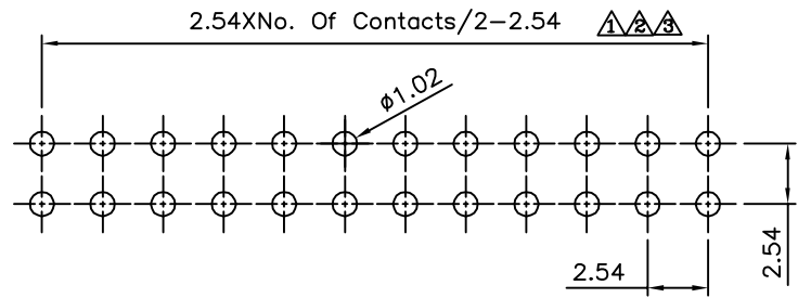
Recommended P.C.B. Layout PCB Tolerance: ±0.05 (Top View)
