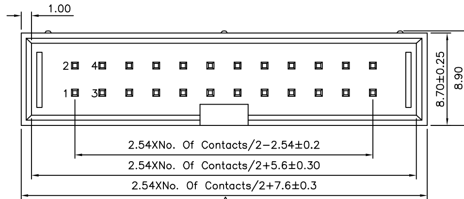
Recommended P.C.B. Layout PCB Tolerance: ±0.05 (Top View)
